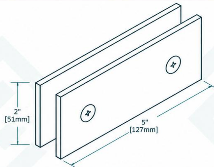
Template For 180° Glass to Glass Clip
