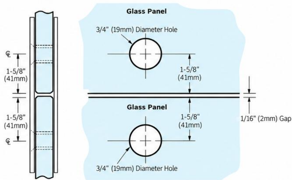
Template For 180° Glass to Glass Clip
